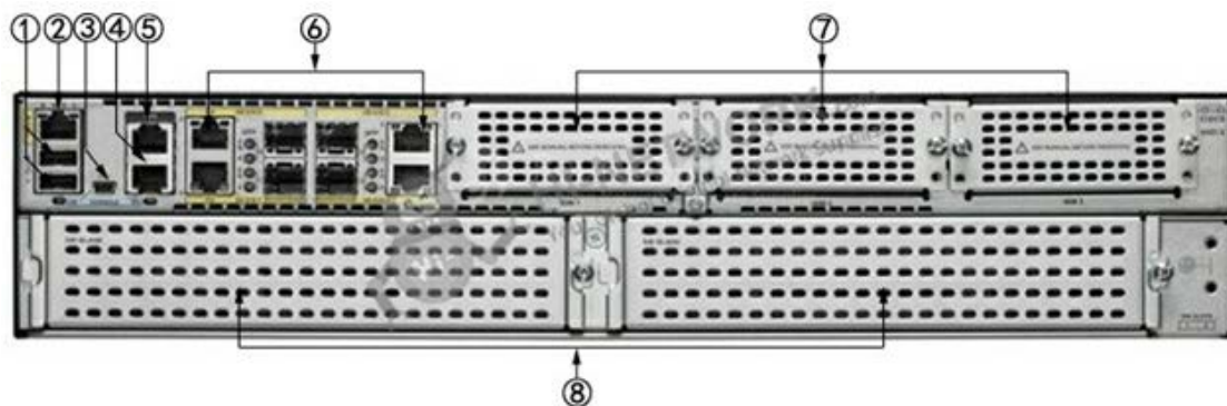
Figure 3 shows the back panel of Cisco ISR4451-X-SEC/K9.
