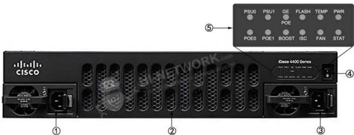
Figure 2 shows the front panel of Cisco ISR4451-X-SEC/K9.
