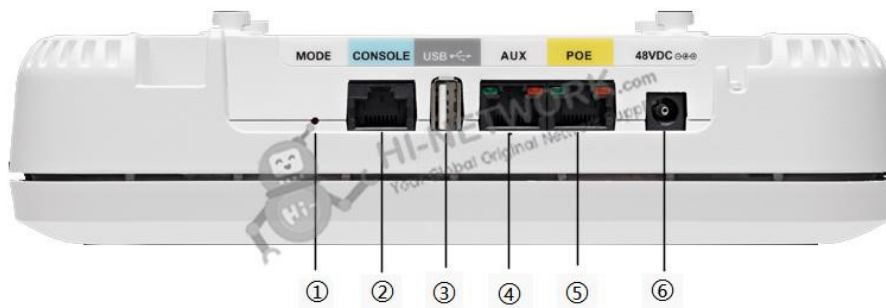
Figure 2 shows AIR-AP1852E Ports and Connections.
