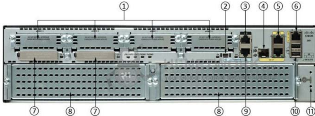
Figure 2 shows the ports on the back panel of CISCO2921-SEC/K9
